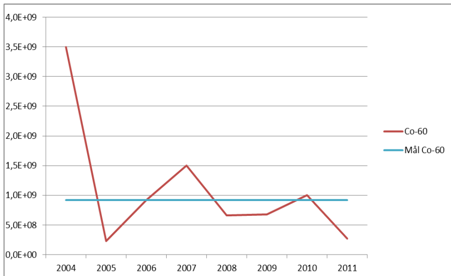
Figure 3.10a Release of Co-60 from R1
