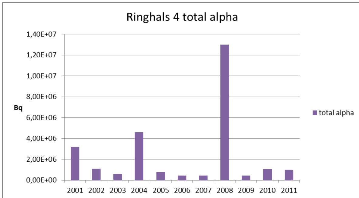
Figure 3.4B Discharges in Bq from Ringhals Unit 4, 2001-2007, for total alpha
