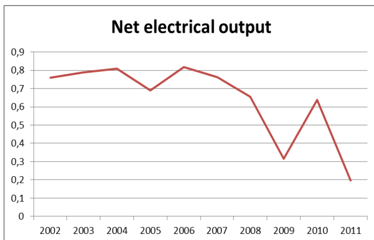
Figure 3.7c Net electrical output (GWa) from Ringhals 2
