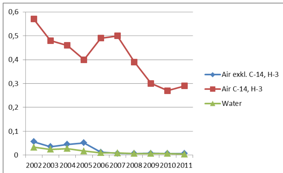
Figure 3.11 Annual effective dose (microSv) to members of the critical group around Ringhals
