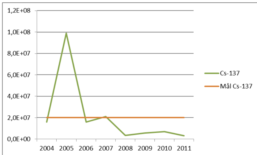
Figure 3.10b Release of Cs-137 from R2
