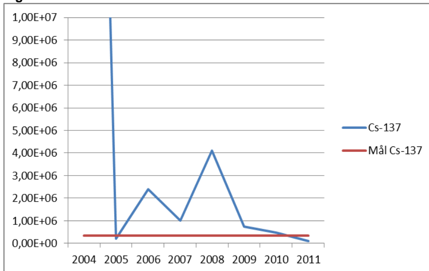
Figure 3.10d Release of Cs-137 from R4
