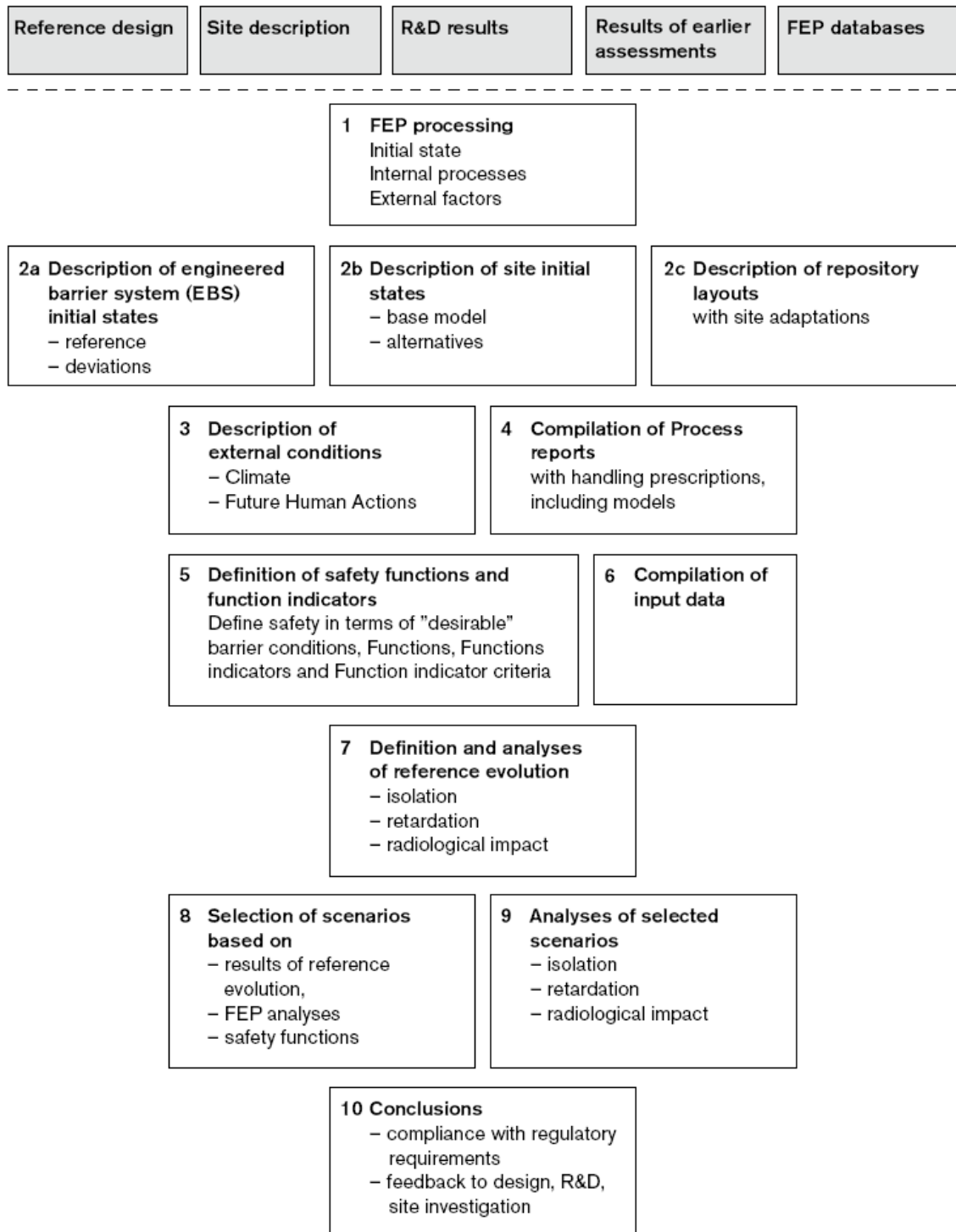
Figure 2: An outline of the 10 main steps of the SR-Can Safety Assessment Methodology. The boxes at the top above the dashed line are inputs to the assessment (SKB, 2006a)
