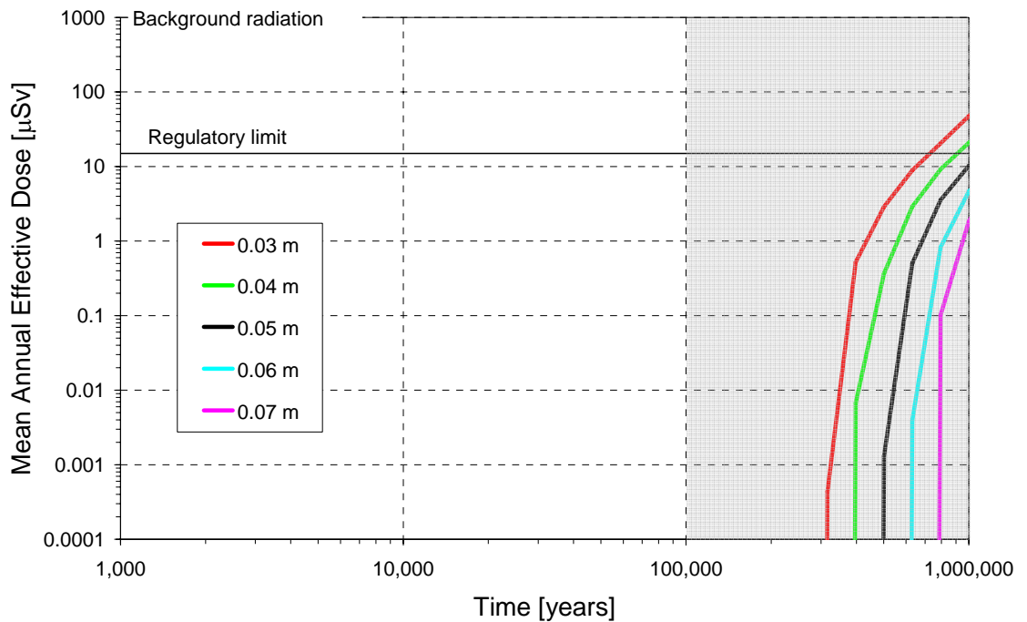
Figure 1. Dose from releases to geosphere for different canister thicknesses. 1,000 realizations of each case, analytical model.
