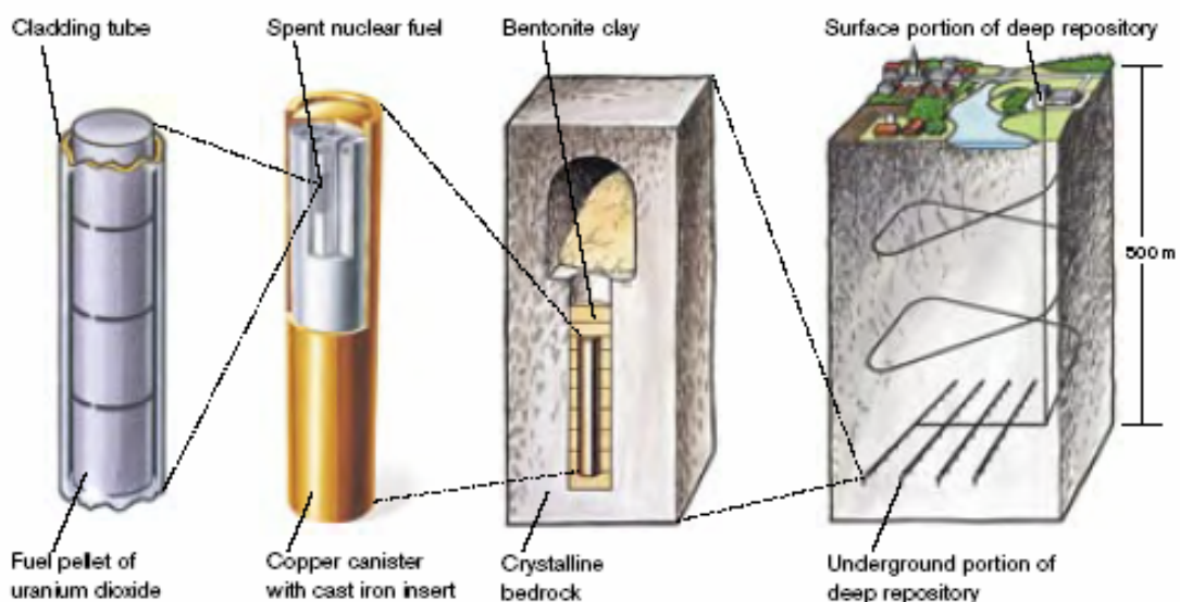
Figure 1: The KBS-3 concept for disposal of spent nuclear fuel (picture from SKB)
