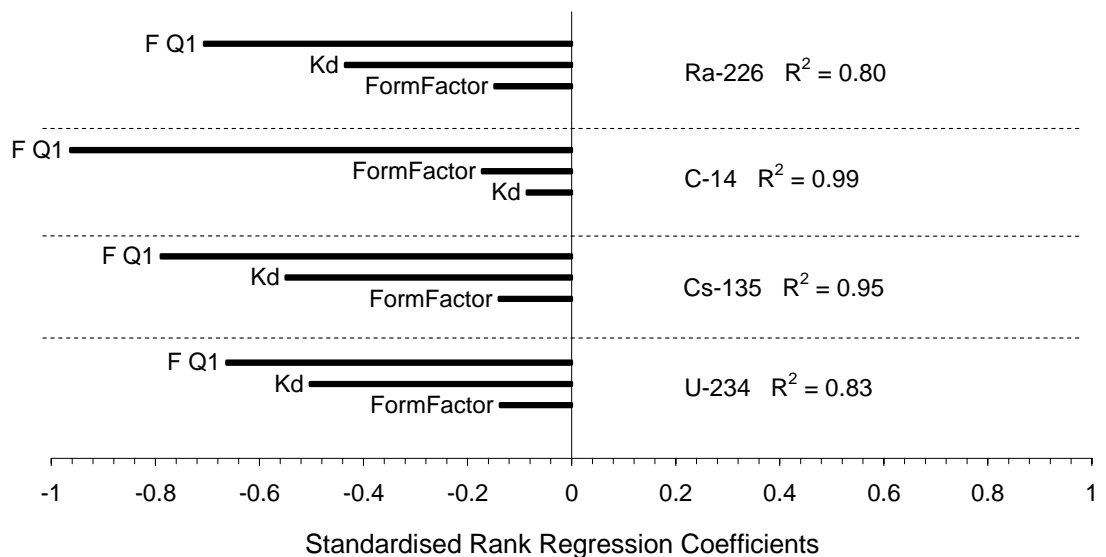
Figure 2. SRRC results for rock transmission at Forsmark.
