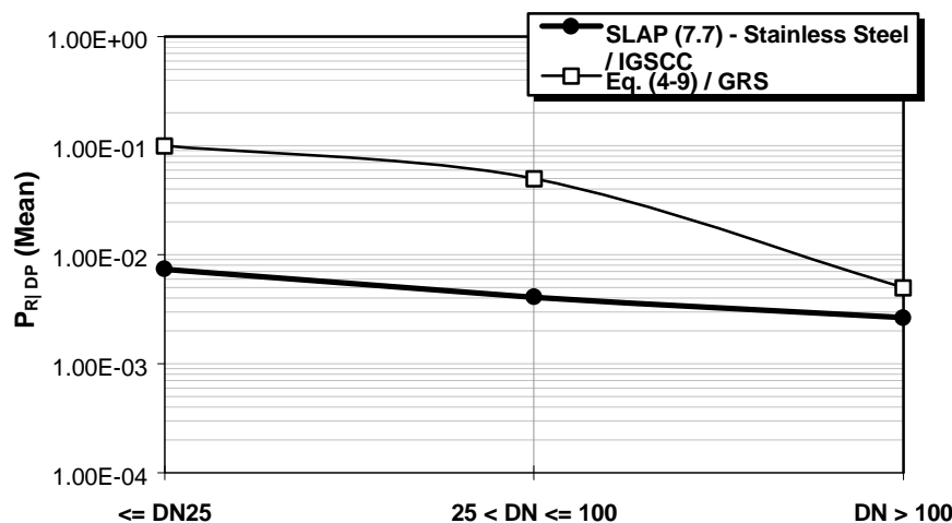
Figure 4-3: Conditional Probability of Pipe Rupture for IGSCC-Susceptible Stainless Steel Piping.
