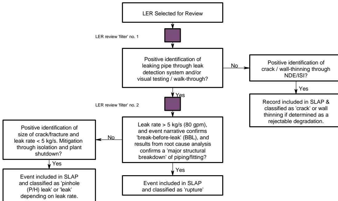
Figure 3-3: Development of the SLAP Database - The Event Review Process.
