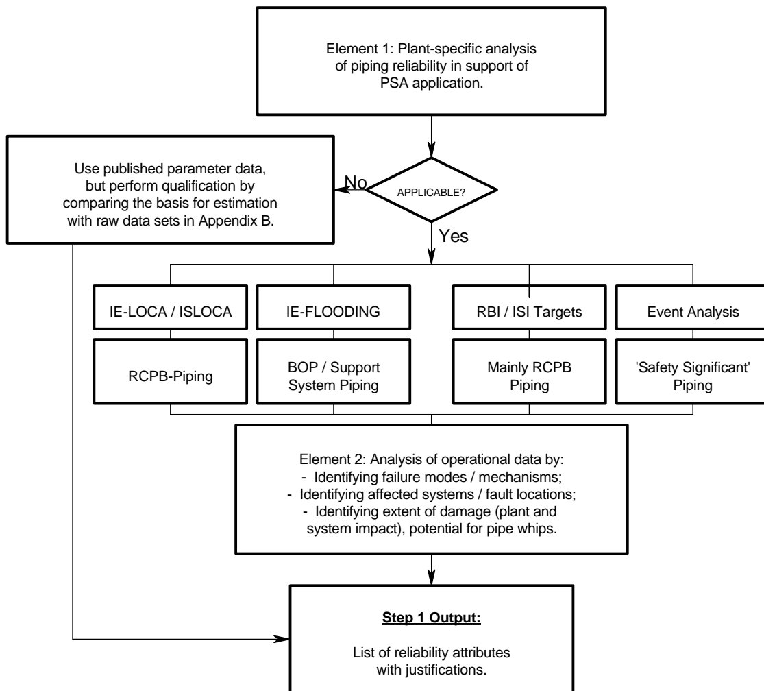
Figure 5-3: Step 1 of the 'PFCA' Framework - Application Requirements.
