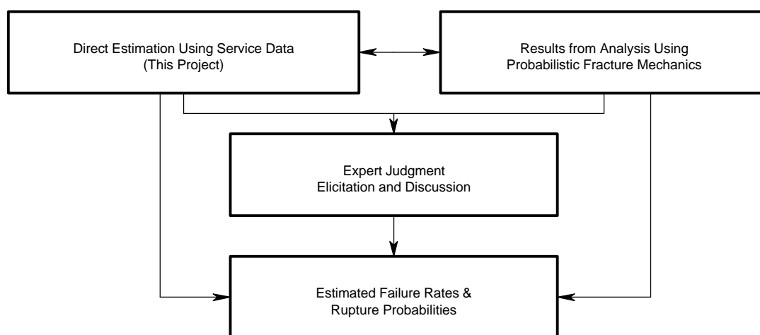
Figure 1-1: The Approaches to Estimating Piping Reliability.
