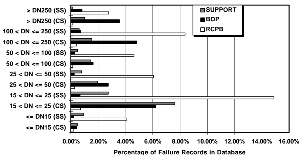
Figure 3-1: Overview of Database Content by System Category 11 .
