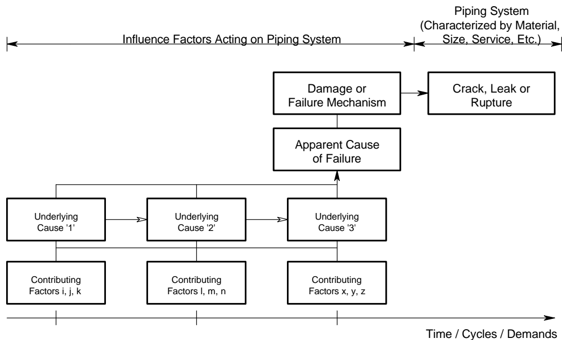
Figure 4-1: Simplified Root Cause Perspective on Attributes and Influences of Piping Failure.
