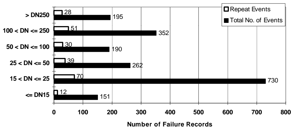
Figure 3-5: Overview of Systematic Failures in the SLAP Database.
