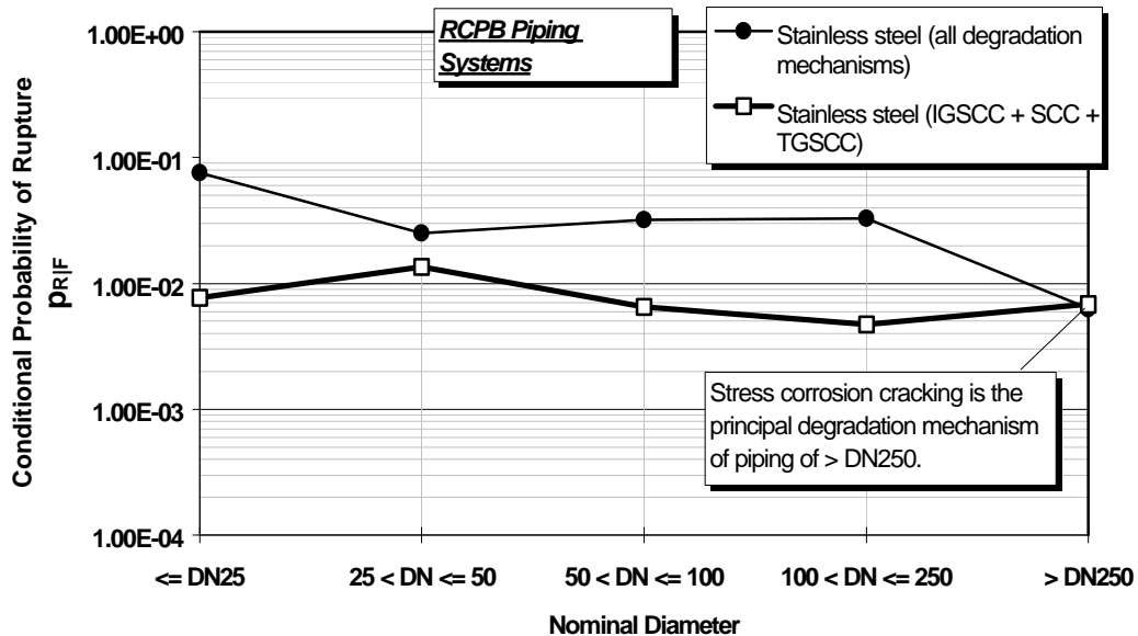
Figure 5-8: Conditional Rupture Probabilities for Different Attributes.
