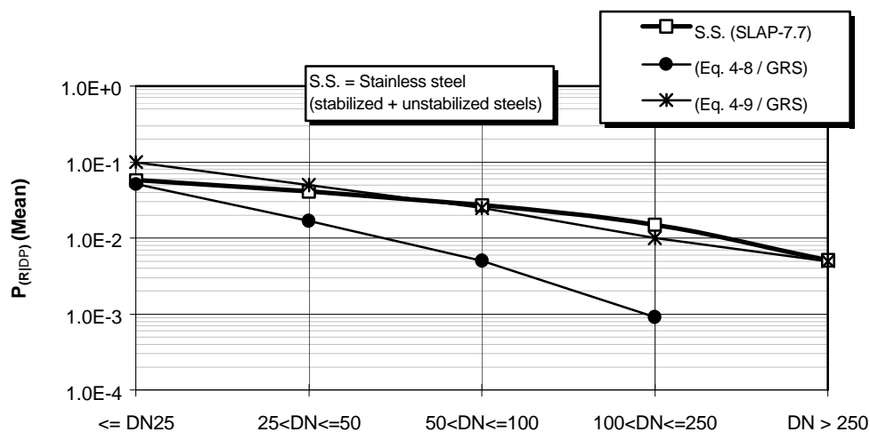
Figure 4-2: The Conditional Probability of Pipe Rupture as a Function of Diameter and Material.
