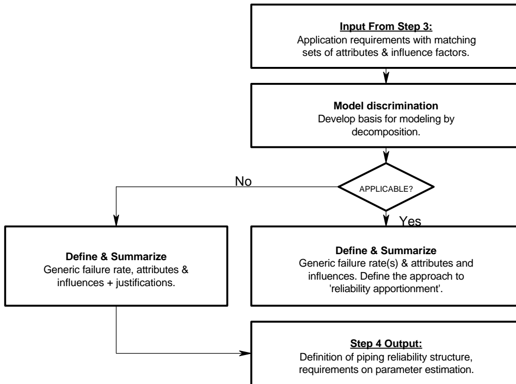
Figure 5-7: ‘Step 4 of the PFCA’ Framework - Estimation of Pipe Rupture Frequency.
