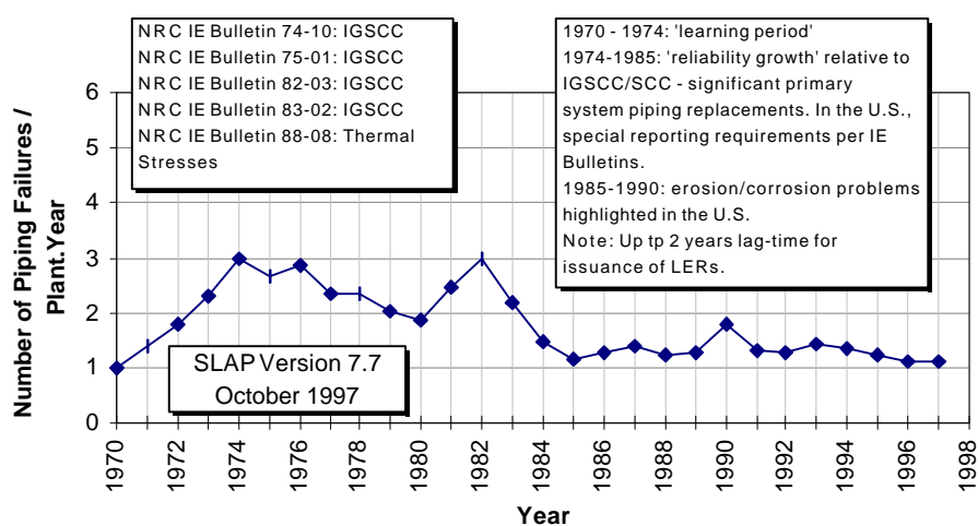
Figure 3-4: The SLAP Database Content - Number of Failures per Plant and Year.
