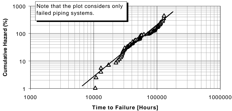
Figure 4-5: Hazard Plot 17 - Leaks in Stainless Steel Piping in BWR Due to IGSCC (4-17) .
