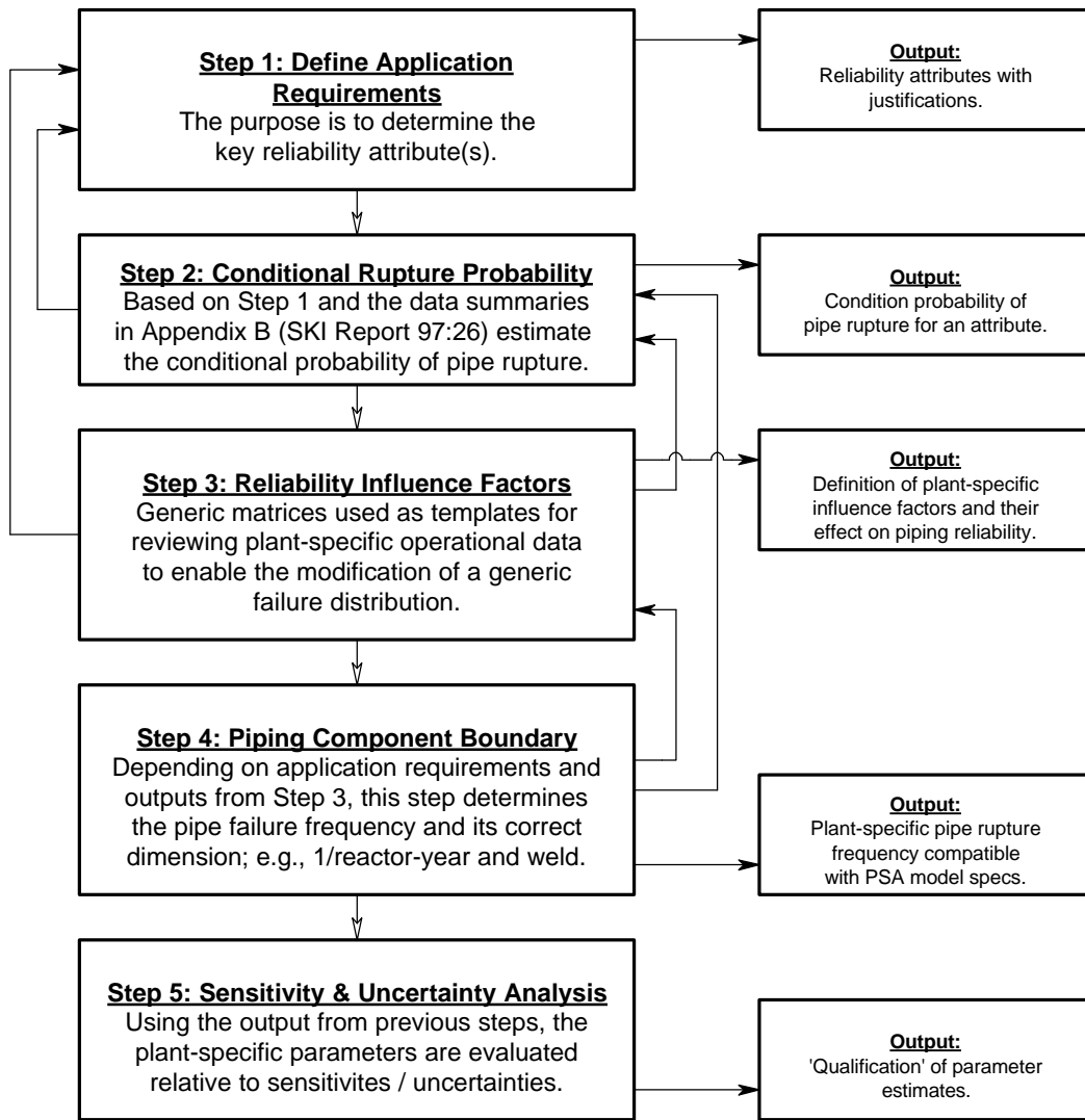
Figure 1-2: The Five-Step PFCA Framework for Piping Reliability Analysis.
