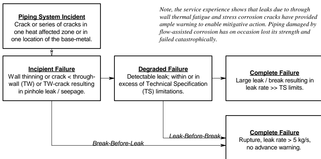
Figure 3-2: Pipe Failure Mode Definitions Used in Developing the SLAP Database.
