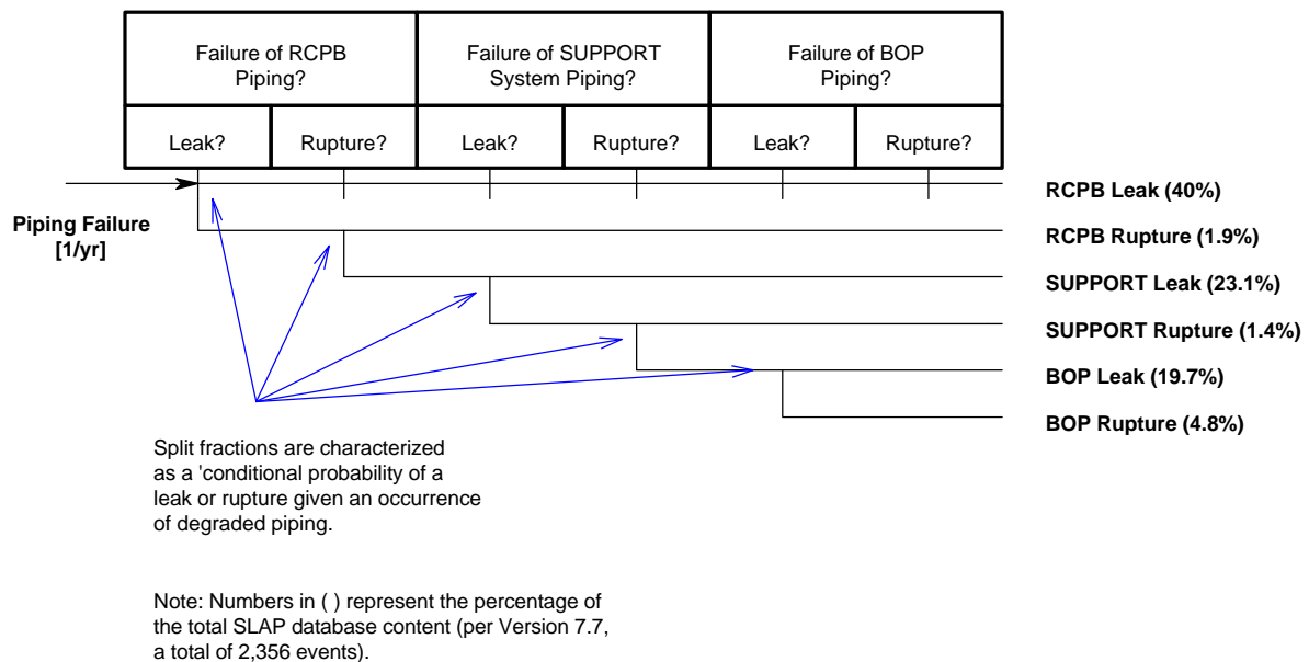
Figure 5-2: Illustration of the Data Needs - The Frequency of Pipe Failure.
